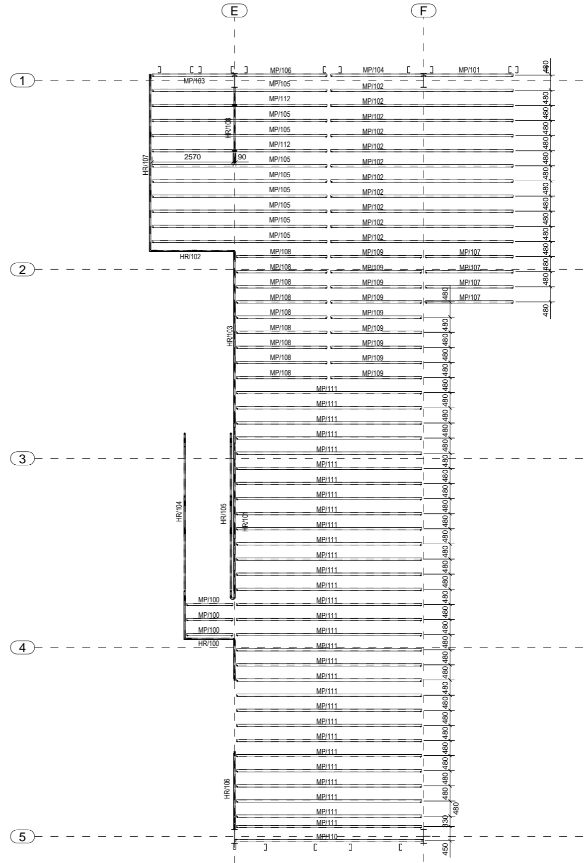
PURLIN & RAIL MARKING PLAN
